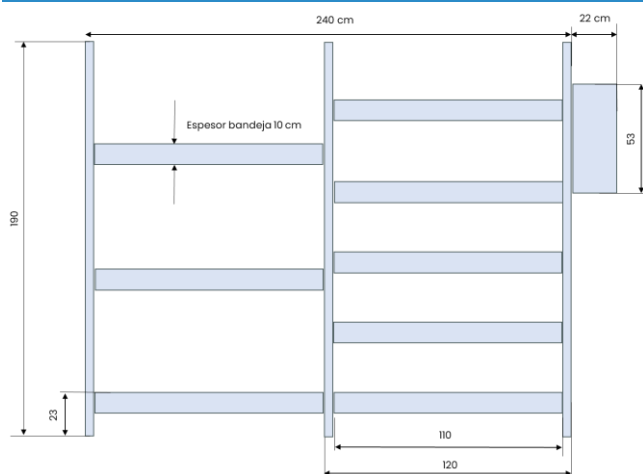
Front view Double Skalex Shelving
