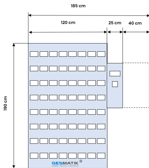
Front View Skalex Cabinet
