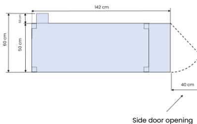
Top View Skalex Shelving
